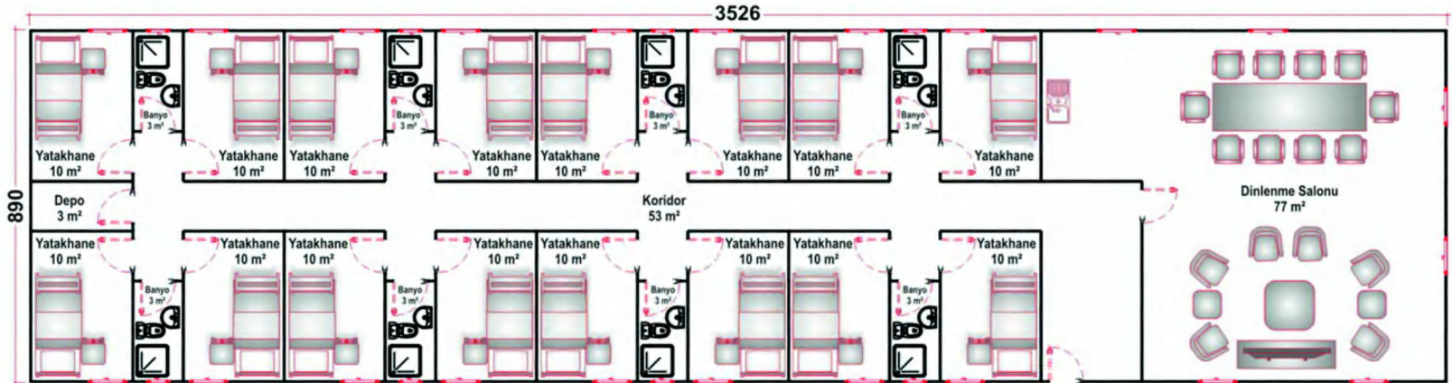
• 314 m 2 Prefabrik Yatakhane
