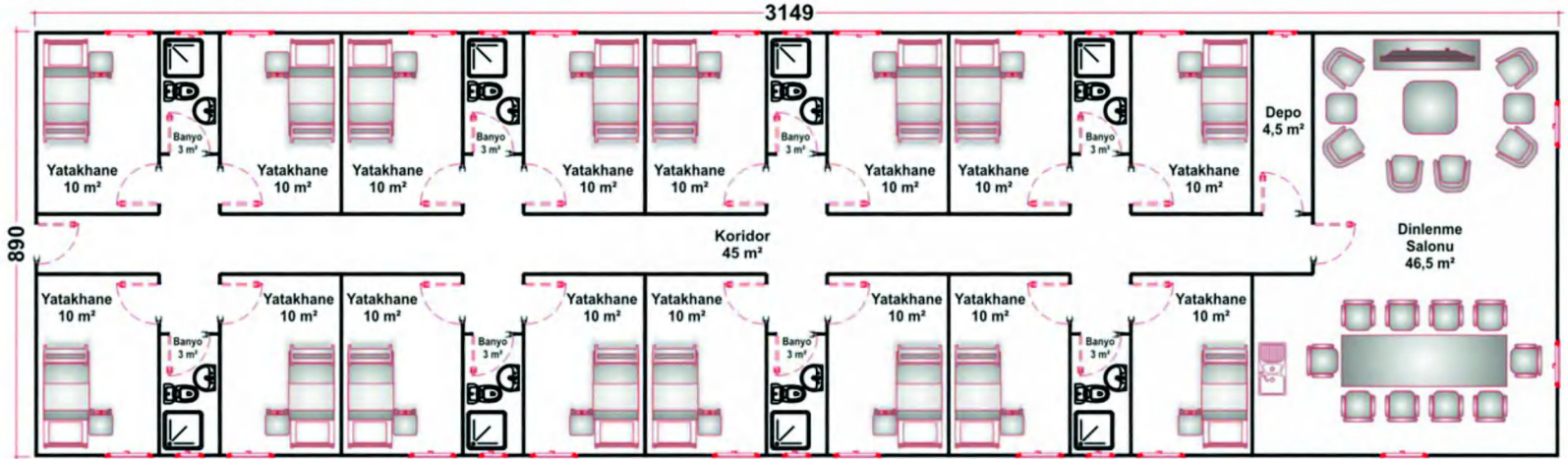
• 280 m 2 Prefabrik Yatakhane
